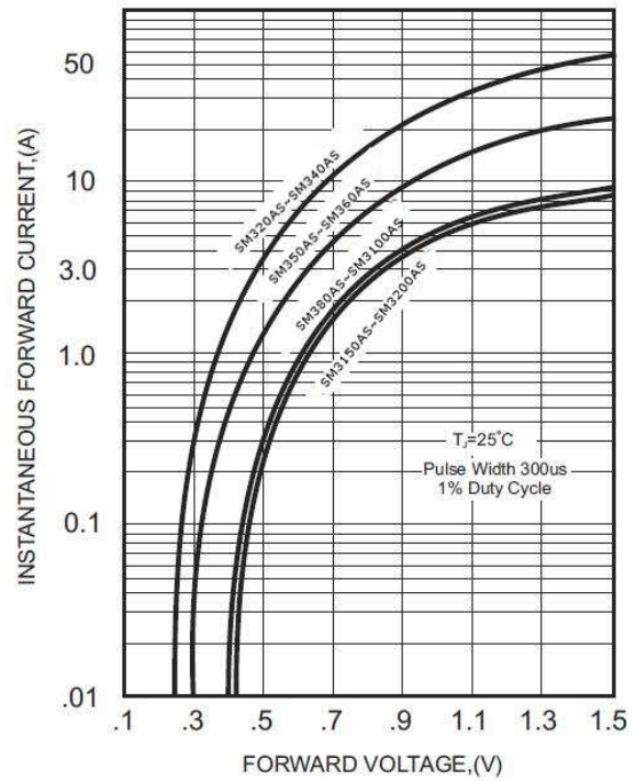
FIG.2-TYPICAL FORWARD CHARACTERISTICS
